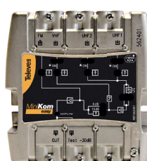
Centralino Minikom EasyF FM+VHF+UHF+UHF: 114/117dBuV Guadagno: 40dB cod. 562401
